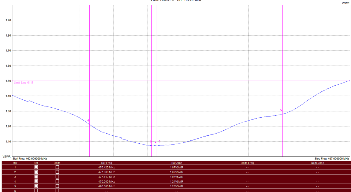
Typical VSWR
