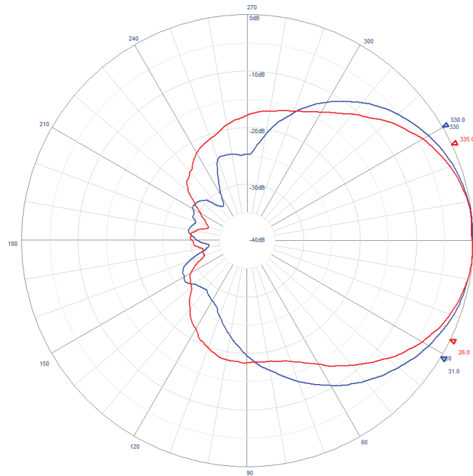
Example radiation pattern - RA4-R
