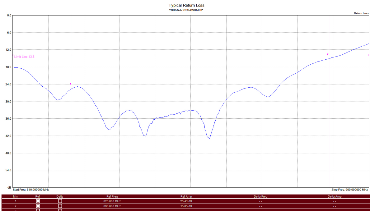
Typical Return Loss - Y806A-R
