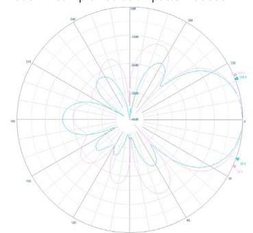
Y806A-R Sample Radiation pattern at 880MHz
