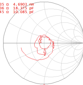
Typical VSWR
