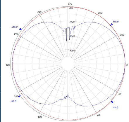
B205BSS Radiation Pattern
