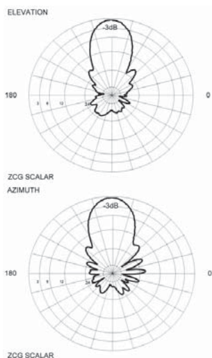
Y415 fitted with YFRS-AL Flat Rear Screen
