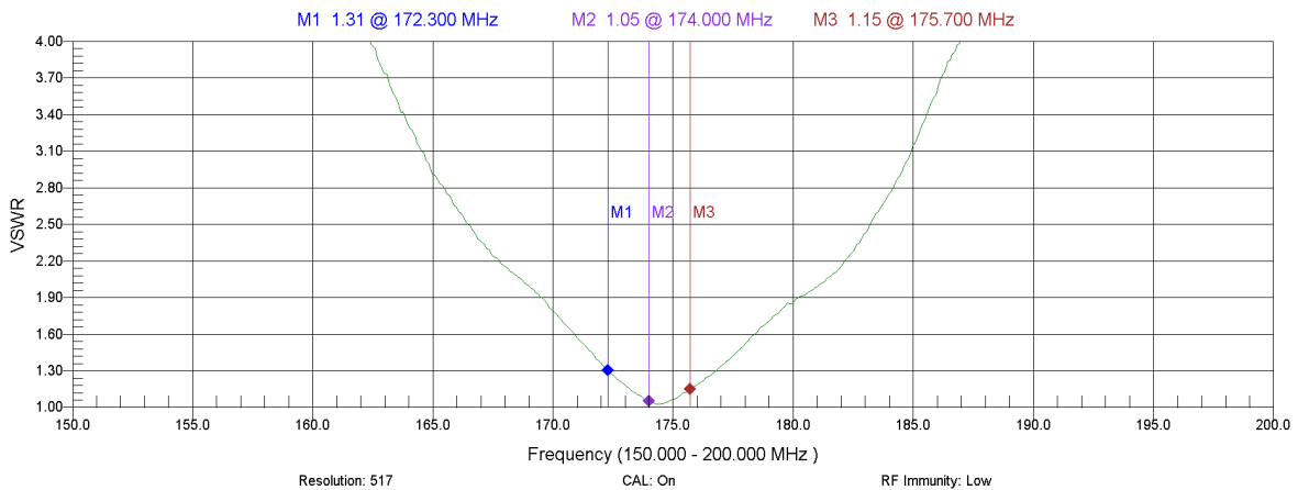
Typical VSWR - from factory
