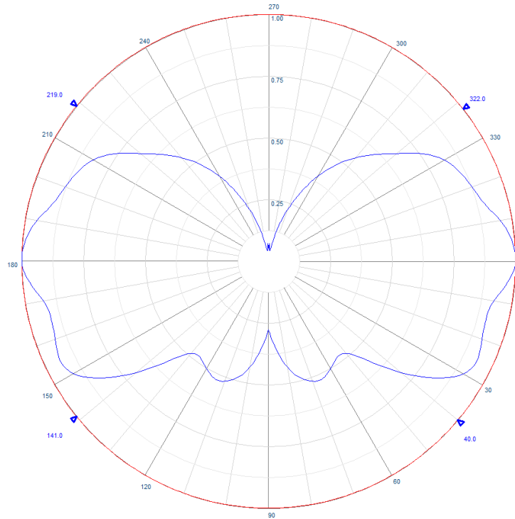
Example polar radiation pattern
