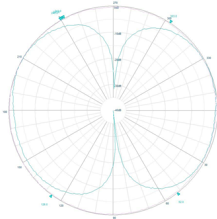
Example radiation pattern at 148MHz on metallic 1/4 wave ground plane
