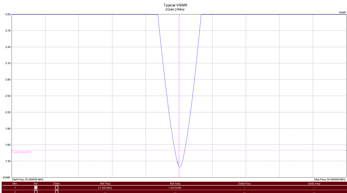
Typical VSWR - ZGI40
