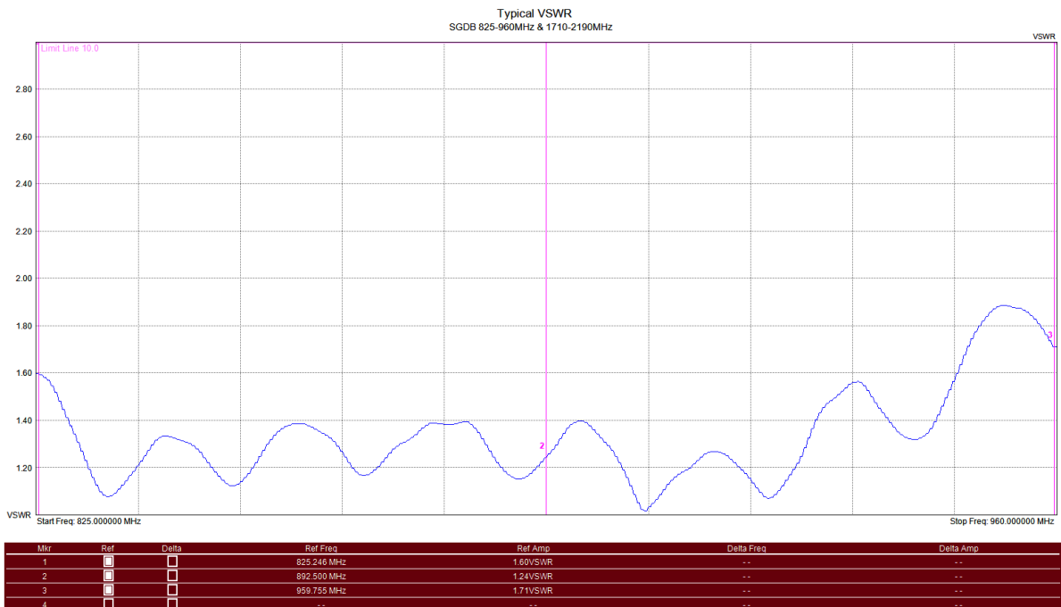
Typical VSWR
