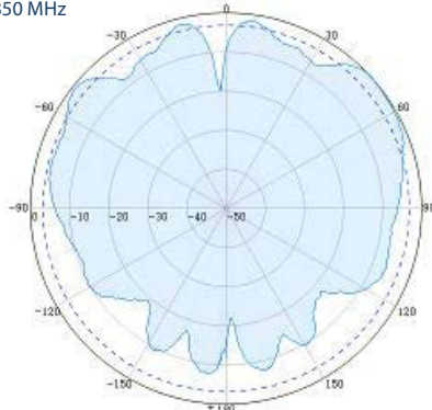
Vertical @ 5850 MHz
